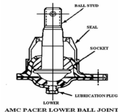
AMC PACER LOWER BALL JOINT
