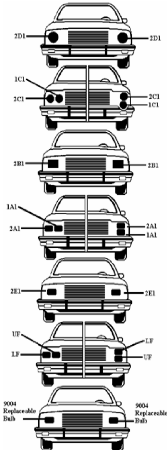
Locations of Type 1, Type2, LF/UF, and Replaceable Bulb Headlamps
