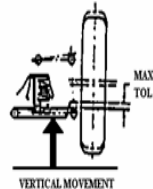
RAISING POSITIONS FOR SUSPENSION SYSTEMS
