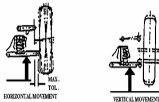
RAISING POSITIONS FOR SUSPENSION SYSTEMS
